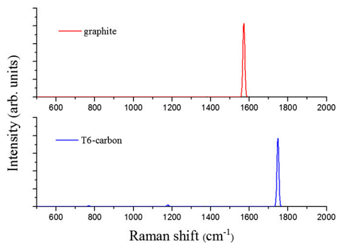
Fig. S2. Calculated first-order Raman spectra of graphite and T6-carbon. Our result in graphite is in good agreement with previous work (1).
