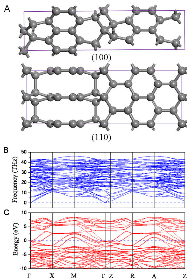
Fig. S3. (A) Optimized geometry of T28-carbon viewed along the [100] and [110] directions, (B) phonon dispersions, and (C) electronic band structure of T28-carbon.
