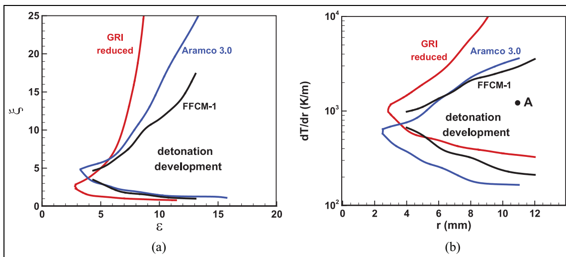
Figure 6. Detonation development regimes predicted by different kinetic models for a stoichiometric \text{CH}_4/\text{air} mixture initially at T_0 = 1300 \text{ K} and P_0 = 40 \text{ atm} in the plots of (a) \xi-\epsilon and (b) dT/dr-r . Point A corresponds to (dT/dr)_0 = -1050 \text{ K/m} and r_0 = 11 \text{ mm} .
