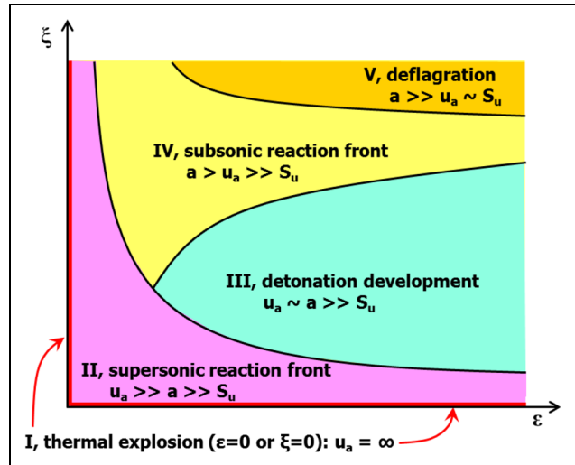
Figure 1. Schematics of different regimes of autoignitive reaction front propagation induced by a hot spot (figure from Gao et al. 30 ). Five modes, I–V, are determined based on the comparison among difference characteristic speeds.
