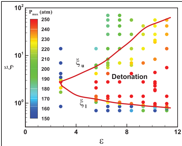
Figure 5. Maximum pressure and detonation regime predicted by the reduced GRI mechanism for a stoichiometric \text{CH}_4/\text{air} mixture initially at T_0 = 1300 \text{ K} and P_0 = 40 \text{ atm} .
