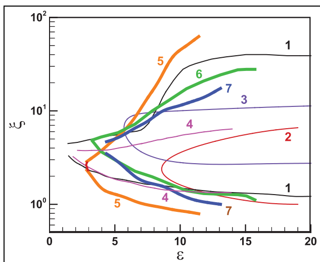
Figure 8. The detonation regime in the \xi - \varepsilon diagram for different stoichiometric fuel/air mixtures: line #1 for \text{H}_2/\text{CO}/\text{air} at T_0 = 1000\text{ K} and P_0 = 50\text{ atm} , 11 #2 for \text{DME}/\text{air} at T_0 = 1035\text{ K} and P_0 = 40\text{ atm} , 17 #3 for n -heptane/air at T_0 = 802\text{ K} and P_0 = 40\text{ atm} , 17 #4 for toluene reference fuel (42.8% iso-octane, 13.7% n -heptane and 43.5% toluene at T_0 = 1000\text{ K} and P_0 = 50\text{ bar} ; 20 and #5, #6 and #7 for \text{CH}_4/\text{air} at T_0 = 1300\text{ K} and P_0 = 40\text{ atm} , respectively, from reduced GRI mechanism, Aramco 3.0 mechanism and FFCM-1 mechanism (this work).
