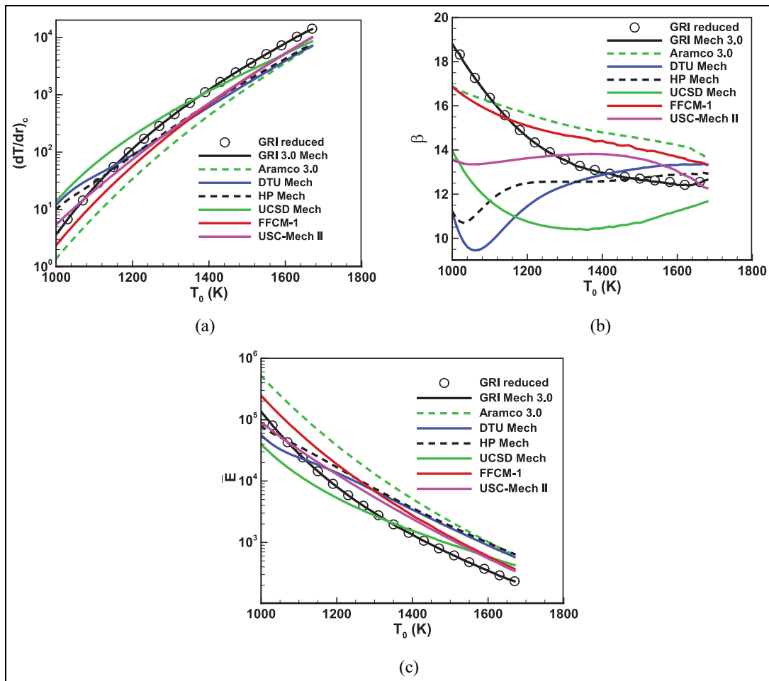
Figure 3. Change in the (a) critical temperature gradient (dT/dr)_c , (b) thermal sensitivity \beta and (c) reduced activation energy \bar{E} with the initial temperature for stoichiometric \text{CH}_4/\text{air} at P_0 = 40 atm.
