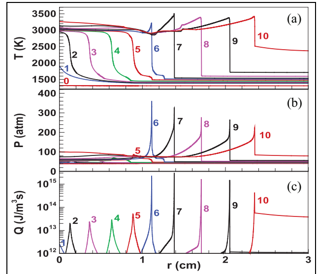
Figure 4. Temporal evolution of the (a) temperature, (b) pressure and (c) heat release rate distributions during the autoignitive reaction front propagation in a stoichiometric \text{CH}_4/\text{air} mixture with a hot spot of r_0 = 9 mm and \xi = 2.8 . The time sequence for lines #0–#10 is 0: 0 \mu\text{s} , 1: 285.5 \mu\text{s} , 2: 288.4 \mu\text{s} , 3: 293.4 \mu\text{s} , 4: 296.4 \mu\text{s} , 5: 299.7 \mu\text{s} , 6: 301.4 \mu\text{s} , 7: 302.8 \mu\text{s} , 8: 304.6 \mu\text{s} , 9: 306.5 \mu\text{s} and 10: 308.2 \mu\text{s} .
