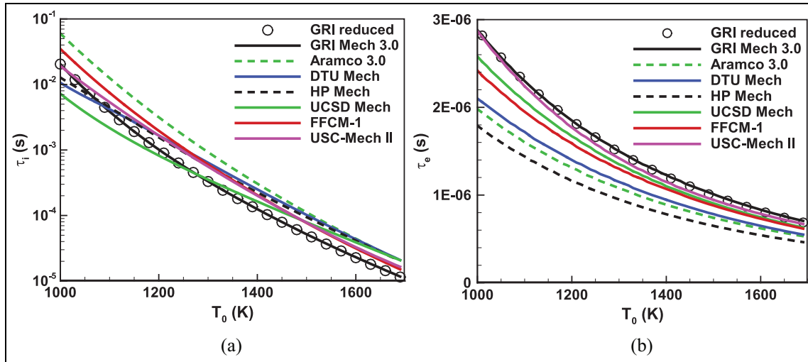
Figure 2. Change in the (a) ignition delay time \tau_i and (b) excitation time \tau_e with the initial temperature for stoichiometric \text{CH}_4/\text{air} at P_0 = 40 atm.
