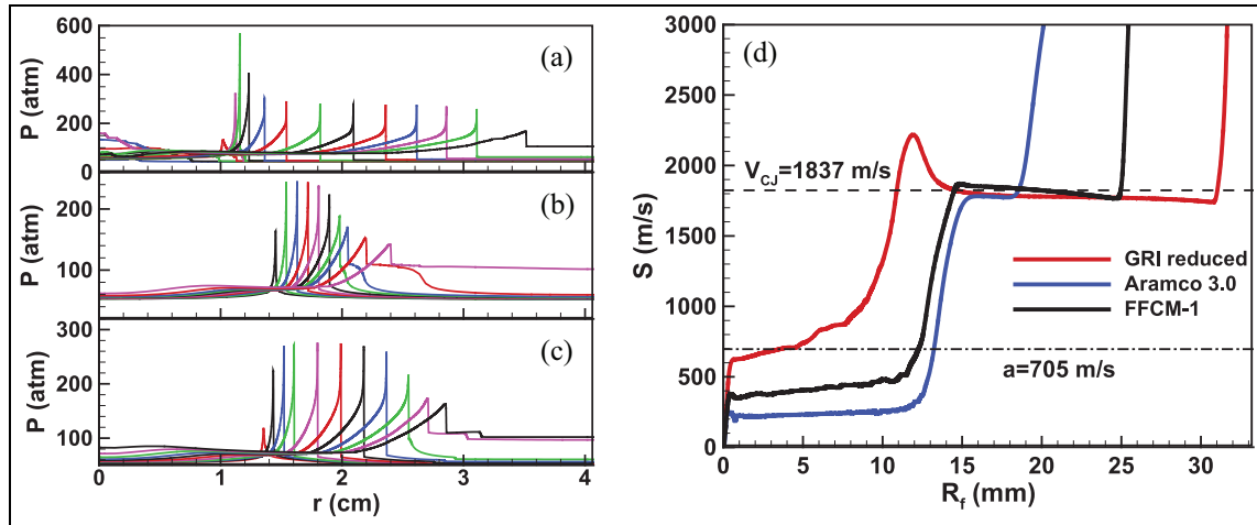
Figure 7. Temporal evolution of the pressure distributions during the autoignitive reaction front propagation from a hot spot with (dT/dr)_0 = -1050 \text{ K/m} and r_0 = 11 \text{ mm} (corresponding point A in Figure 6(b)) predicted by different kinetic models: (a) GRI reduced, (b) Aramco 3.0 and (c) FFCM-1. (d) The reaction front propagation speed S as a function of its location R_f . The CJ detonation speed ( V_{CJ} = 1837 \text{ m/s} ) and sound speed ( a = 705 \text{ m/s} ) are denoted by the horizontal dashed and dashed-dotted lines, respectively.
