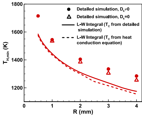
Fig. 8. Change of the critical ignition temperature with hot spot radius for a stoichiometric nC 7 H 16 /air mixture.
