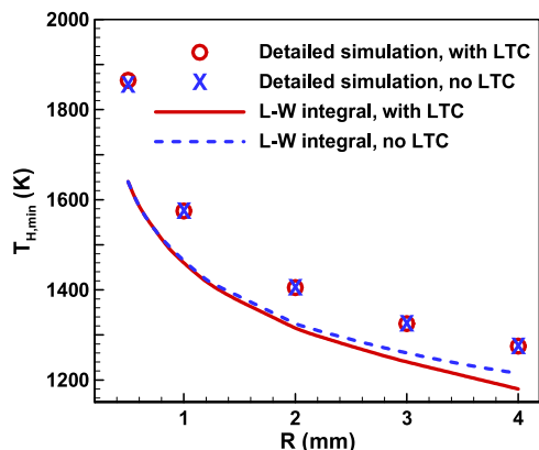
Fig. 12. Effect of low temperature chemistry (LTC) on the critical ignition temperature for a stoichiometric DME/air mixture.
