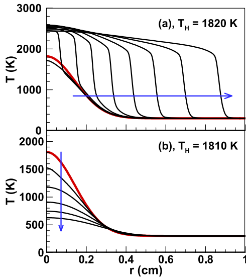
Fig. 1. Evolution of temperature distribution for (a) successful ignition with T_H = 1820 K and (b) ignition failure with T_H = 1810 K in a stoichiometric CH 4 /air mixture with R = 2 mm and M = 2 . The red lines represent initial temperature distributions.
