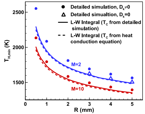
Fig. 6. Change of the critical ignition temperature with hot spot radius for a stoichiometric CH 4 /air mixture. D_k is the mass diffusivity of the species and D_k = 0 ( D_k \neq 0 ) corresponds to the case that the mass diffusivities of all species are artificially set to zero (unchanged).
