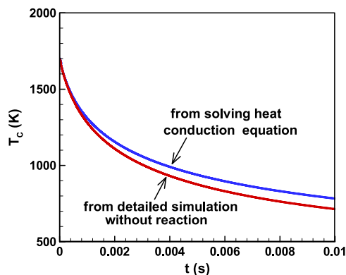
Fig. 3. Change of the central temperature with time in a stoichiometric CH 4 /air mixture with T_H = 1700 K, R = 2 mm and M = 2 .
