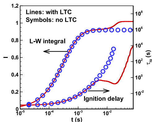
Fig. 11. Effect of LTC on the L-W integral and ignition delay time at the corresponding central temperature from solving the heat conduction equation for a stoichiometric DME/air mixture with T_H = 1320 K, R = 2 mm and M = 2 .
