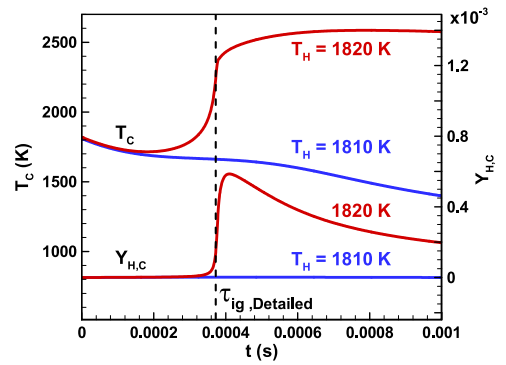
Fig. 2. Change of the central temperature and H mass fraction with time for two cases considered in Fig. 1.
