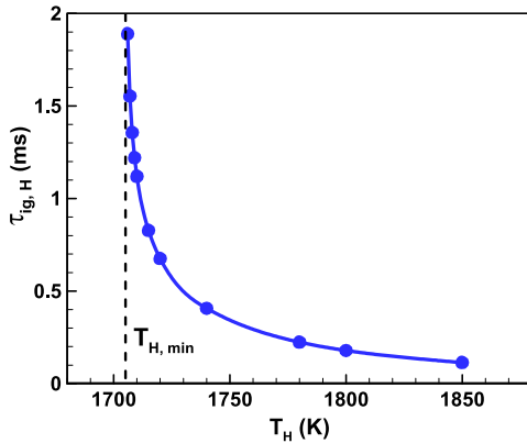
Fig. 5. Change of the ignition delay with hot spot temperature in a stoichiometric CH 4 /air mixture with R = 2 mm and M = 2 . The vertical dashed line represents the minimum hot spot temperature for successful ignition.
