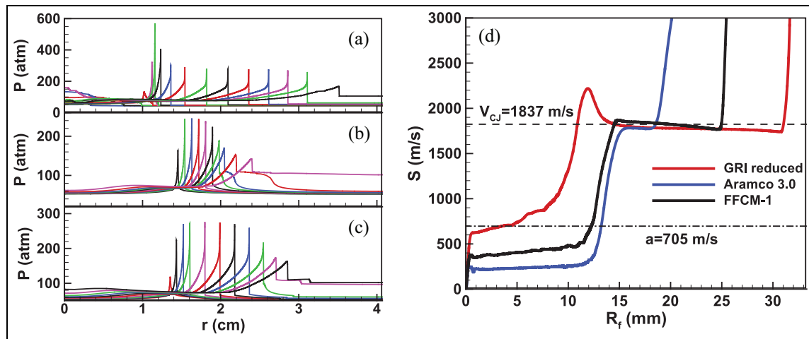
Figure 7. Temporal evolution of the pressure distributions during the autoignitive reaction front propagation from a hot spot with (dT/dr)_0 = -1050 K/m and r_0 = 11 mm (corresponding point A in Figure 6(b)) predicted by different kinetic models: (a) GRI reduced, (b) Aramco 3.0 and (c) FFCM-1. (d) The reaction front propagation speed S as a function of its location R_f . The CJ detonation speed ( V_{CJ} = 1837 m/s) and sound speed ( a = 705 m/s) are denoted by the horizontal dashed and dashed-dotted lines, respectively.
