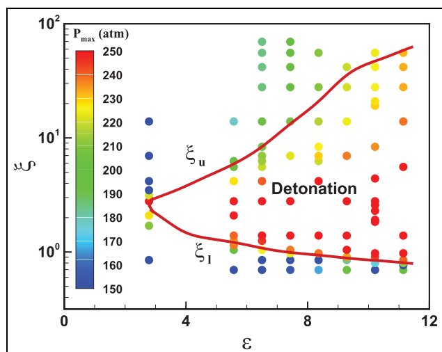
Figure 5. Maximum pressure and detonation regime predicted by the reduced GRI mechanism for a stoichiometric \text{CH}_4/\text{air} mixture initially at T_0 = 1300 \text{ K} and P_0 = 40 \text{ atm} .
