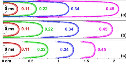
Fig. 7. Sequences of temperature contour lines from 1200 K to 1800 K for different initial temperatures: (a) T_0=100 K, (b) T_0=200 K, and (c) T_0=300 K. See also the animation in the Supplementary Material.
