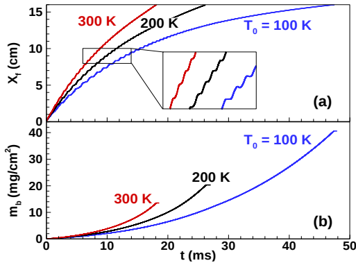
Fig. 3. Temporal evolution of (a) flame position, X_f , and (b) mass of burned gas, m_b , for different initial temperatures.
