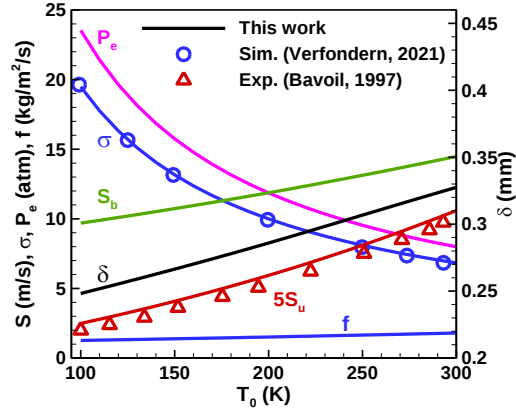
Fig. 2. Properties of steady, planar, premixed H_2 /air flames at atmospheric pressure and different initial temperatures. S_u and S_b are laminar flame speed relative to the unburned and burned gas, respectively. f=\rho_u S_u is the laminar burning flux, \delta the flame thickness, \sigma the expansion ratio, and P_e the equilibrium pressure. The symbols represent laminar flame speeds ( S_u ) measured in experiments and the expansion ratio ( \sigma ) calculated using a real gas equation of state reported in [3, 22].
