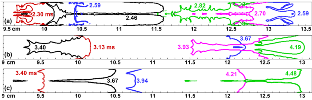
Fig. 10. Temporal evolution of the flame front for (a) T_0=100 \text{ K} , (b) T_0=200 \text{ K} and (c) T_0=300 \text{ K} . See also the animation in the Supplementary Material.
