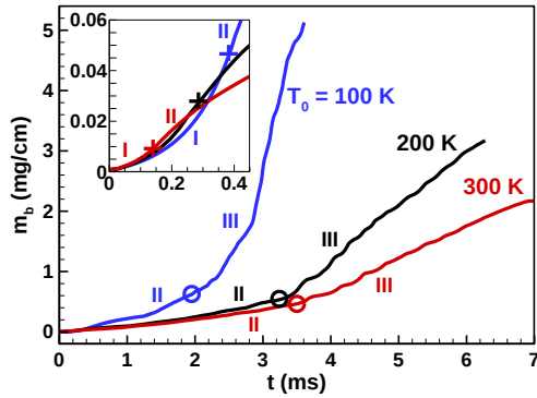
Fig. 5. Change of the burned mass with time. The symbol + separates stages I and II, and symbol o separates stages II and III.
