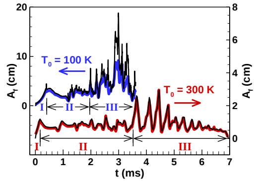
Fig. 6. Change of total flame surface area with time for T_0=100 and 300 K. Thin black lines represent A_f calculated based on Eq. (1) and thick color lines denote A_f based on the iso-surface of T=1000 K. Three stages I, II and III are marked.
