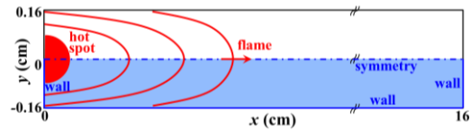
Fig. 1. Schematic of flame propagation in a narrow channel. The computational domain is in blue and the boundary conditions are indicated.
