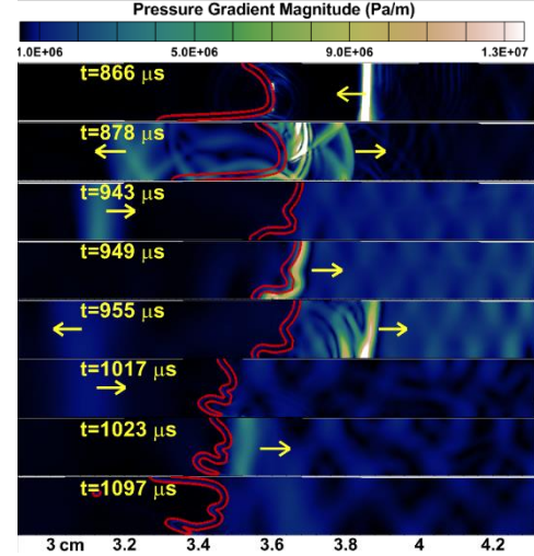
Fig. 8. Temporal evolution of flame-pressure wave interaction for T_0=200 K. Red lines represent the iso-lines of HRR=10^{10} W/m 3 , arrows denote the directions of the pressure wave propagation, and the contour color reflects the magnitude of the pressure gradient. See also the animation in the Supplementary Material.
